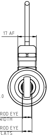
PLUNGER MOUNTED M5 ROD EYE (CODE 'U')
