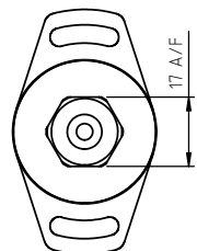
AXIAL IP67 SHORT CABLE GLAND (CODE 'Mxx,MQxx')
